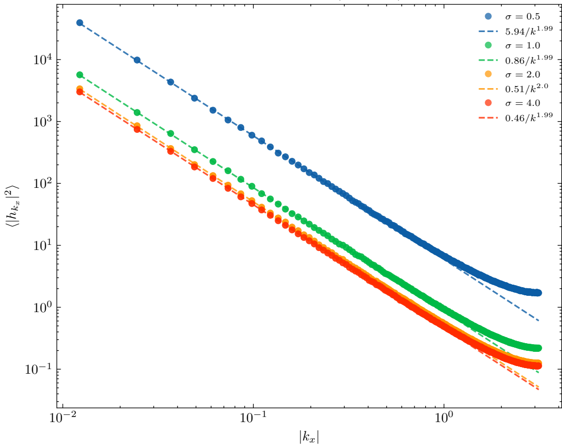
Structure Factor ( L = 512 )
