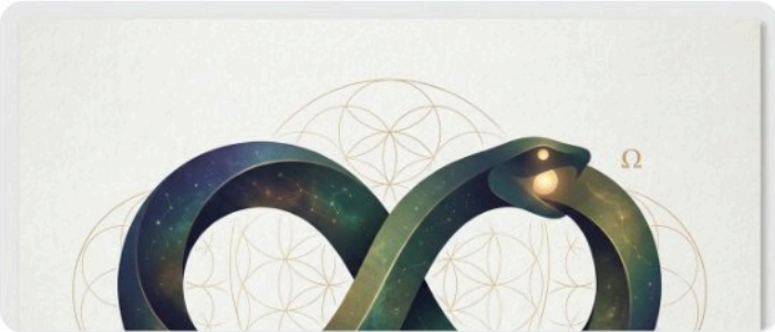
Ouroboros
