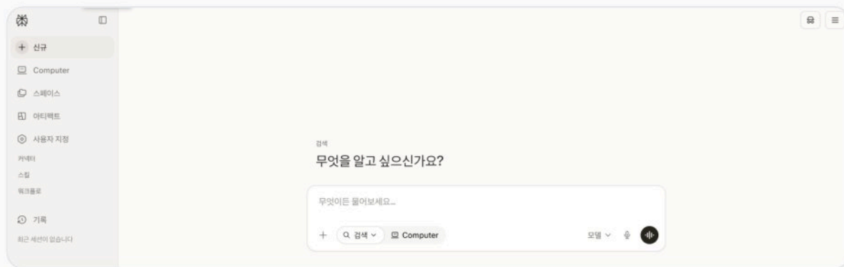
Perplexity
