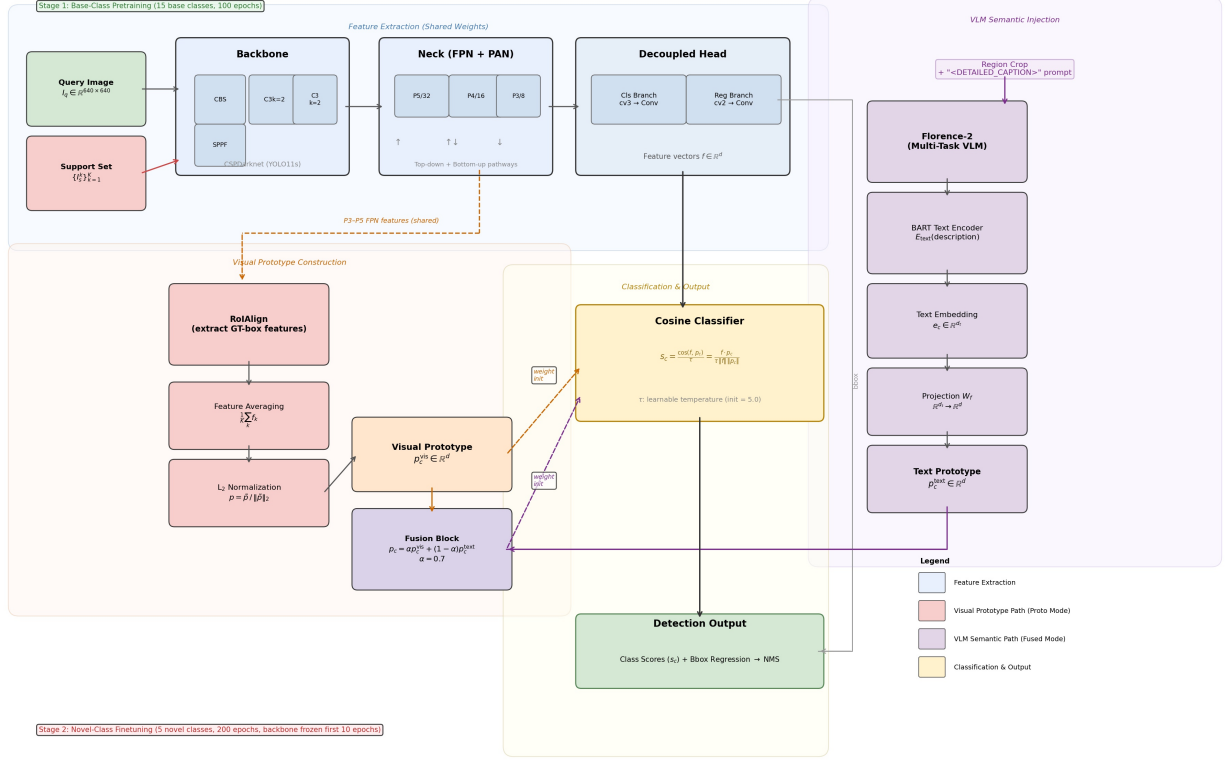
Fig. 1. VCP framework: YOLO11s backbone+neck, decoupled head, cosine classifier. Visual prototypes via RoIAlign; semantic prototypes via Florence-2 + BART. Fused at \alpha = 0.7 .
