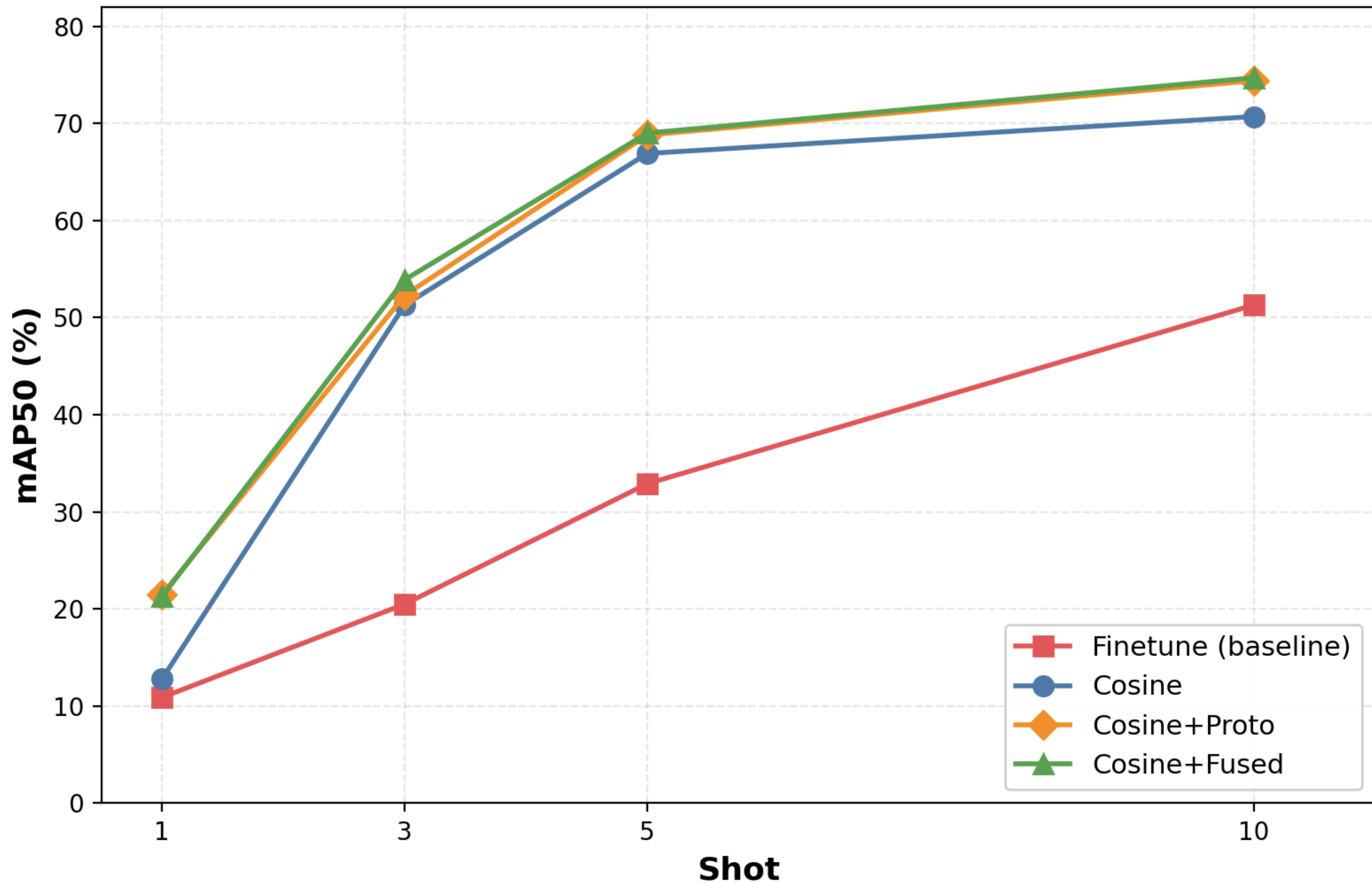
VOC Novel Set mAP50 vs. Shot Count
