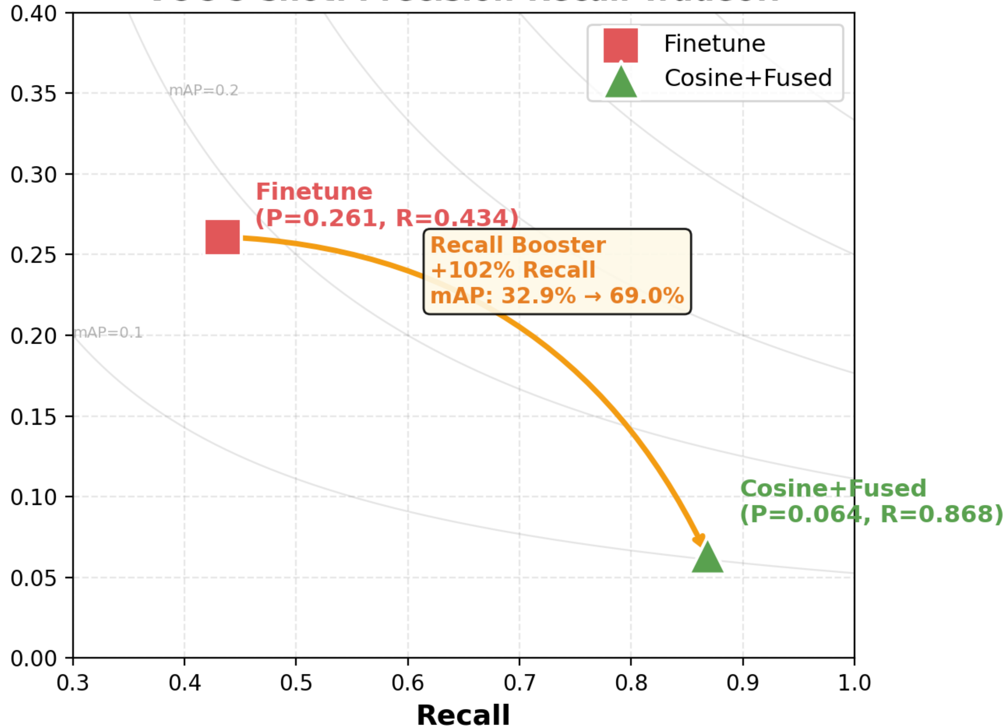
VOC 5-shot: Precision-Recall Tradeoff
