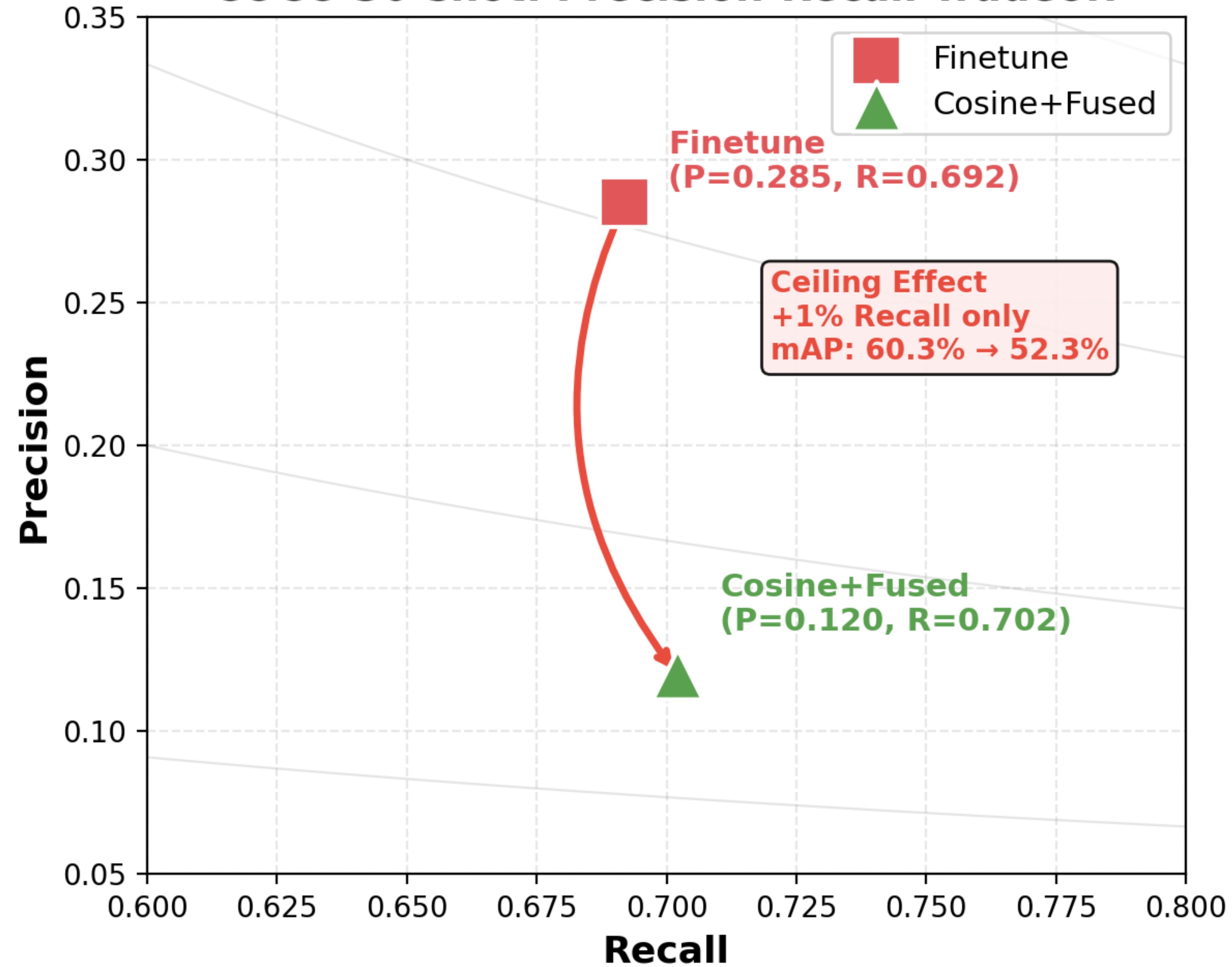
COCO 30-shot: Precision-Recall Tradeoff
