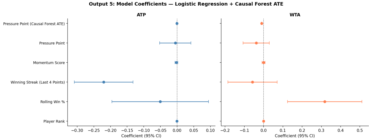
Figure 5: Model results: logistic regression and causal forest estimates
