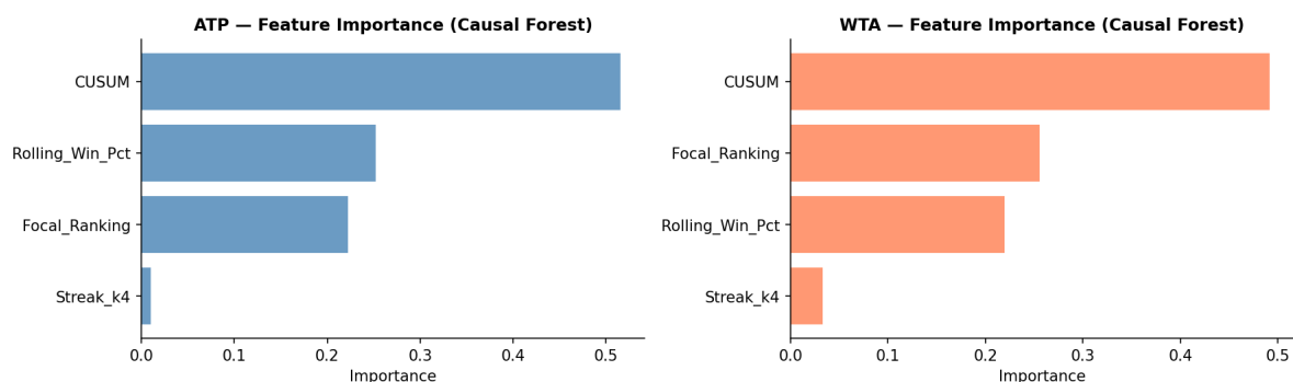
Figure 6: Causal Forest feature importance
