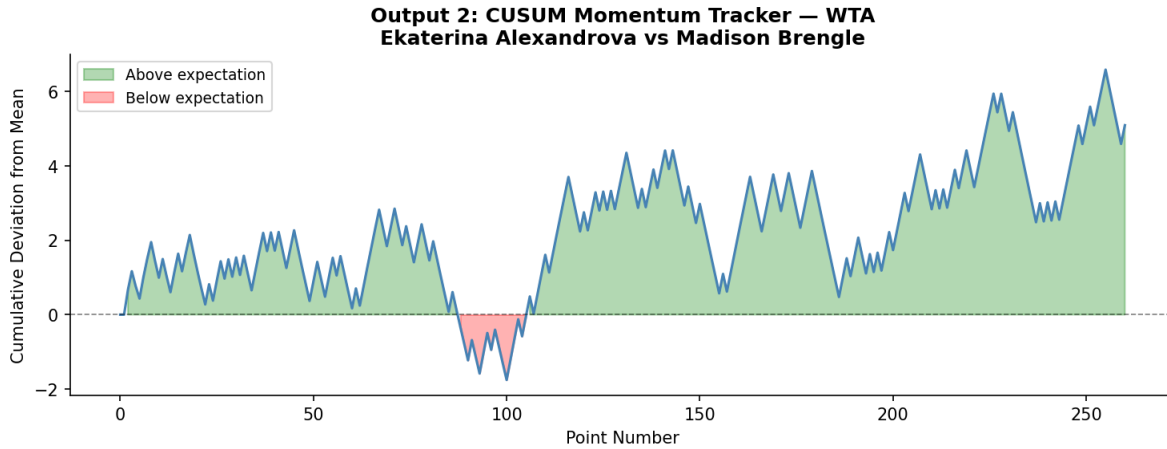
Figure 2: CUSUM momentum tracker, Alexandrova vs Brengle, WTA
