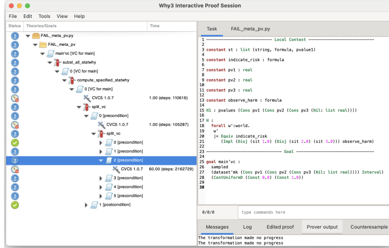
Fig. 5: The Why3 IDE screen showing the failure of verification.
