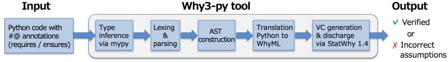
Fig. 1: Overview of the Why3-py verification workflow.
