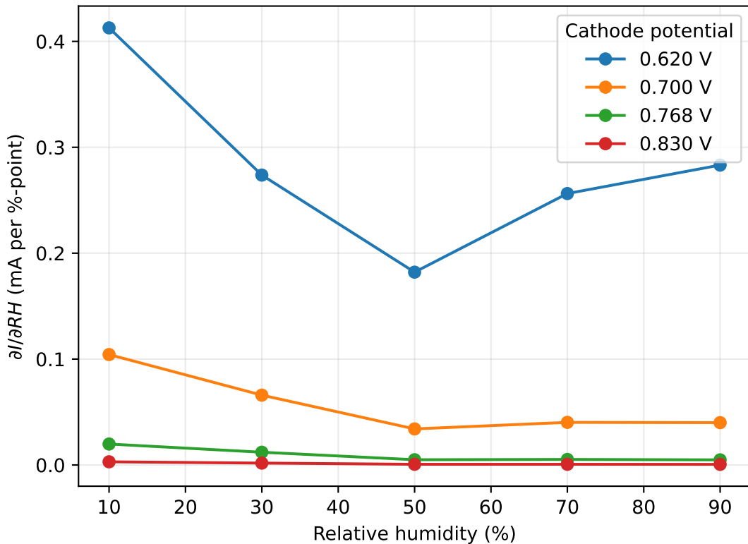
Current sensitivity to cathode relative humidity
