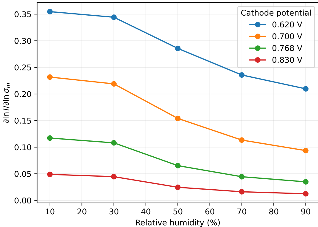
Elasticity of current to protonic conductivity
