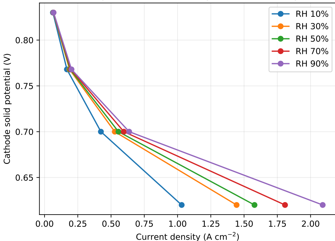
V0.4 polarization curves by relative humidity
