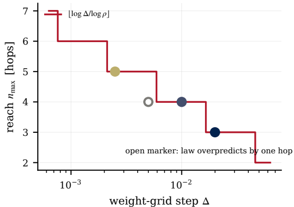
(b) step law, \rho = 0.358 (interior fit)
