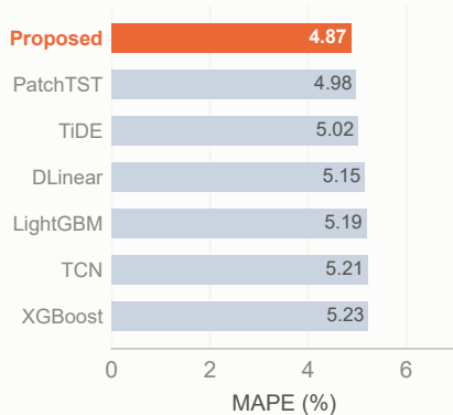
PJM · proposed ranks 1 of 15
