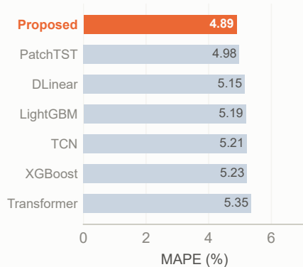
PJM · proposed ranks 1 of 14
