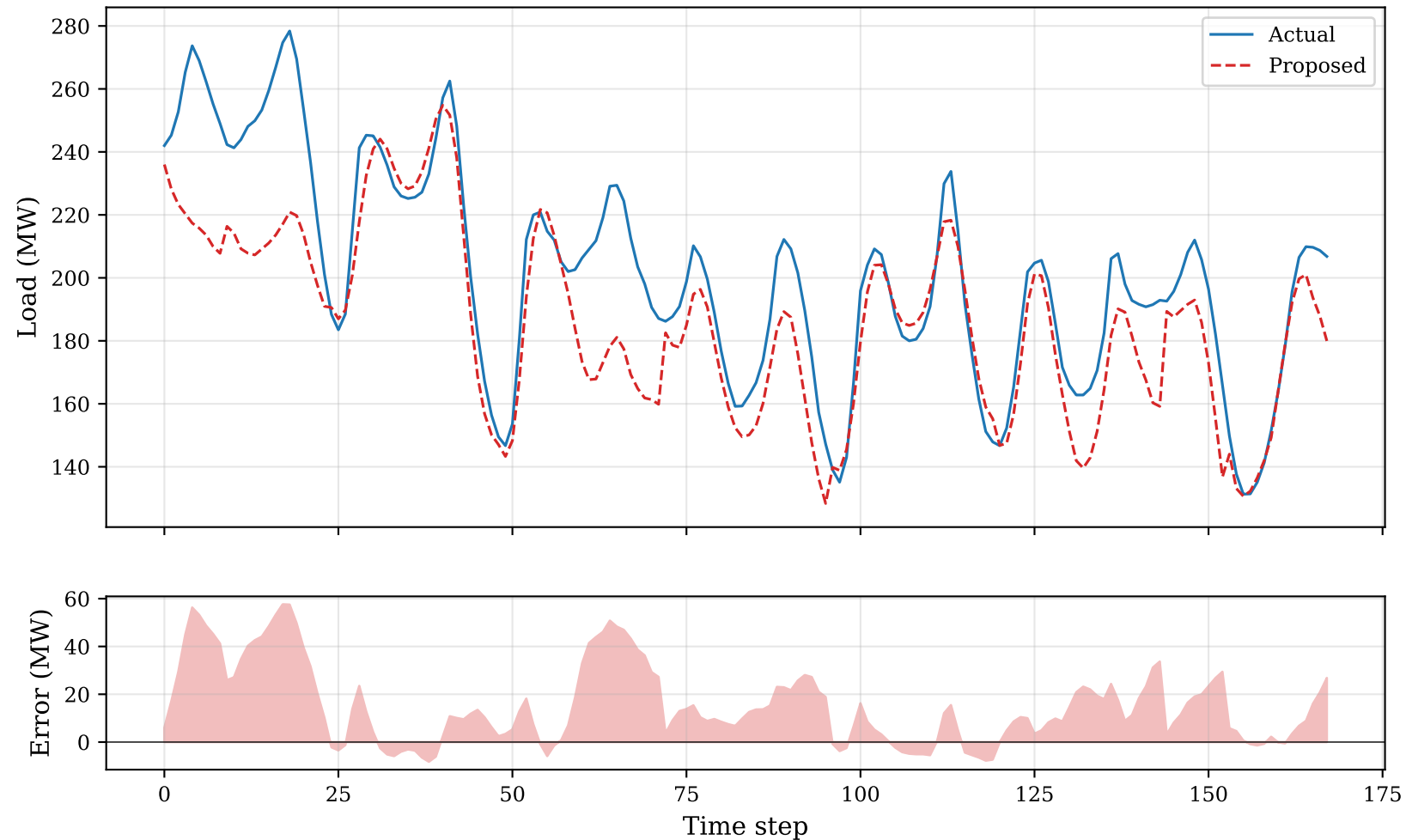
Day-ahead forecasts — GEFCom2014 test set (operational protocol, non-overlapping)
