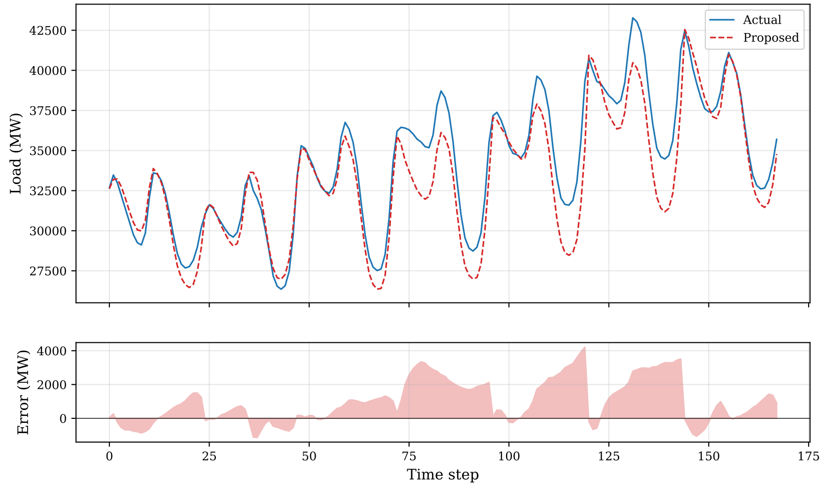
Day-ahead forecasts — PJM test set (operational protocol, non-overlapping)
