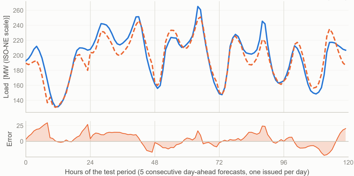
GEFCom2014 — a representative 5-day window · MAPE here 4.58 %, seed-42 test mean 4.58 % (five-seed mean in Table)
