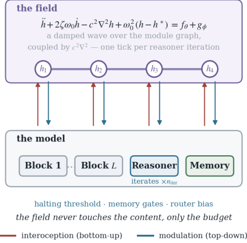
(a) a field layer over the model
