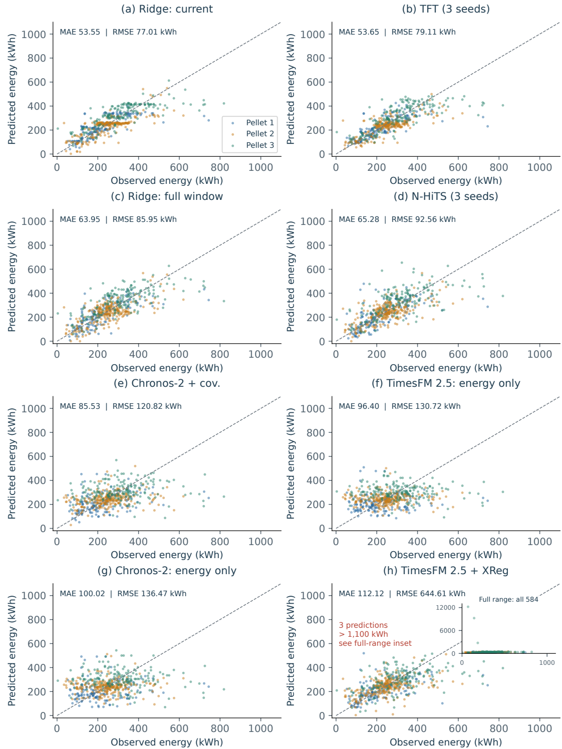
Figure S4: All 4,672 predictions of the matched comparison: eight methods on 584 identical records. Colours identify the three lines and the dashed diagonal marks equality. The main axes share a 0–1,100 kWh range; the TimesFM XReg panel adds a full-range inset containing its three extreme predictions. MAE and RMSE use the complete data in every panel.
