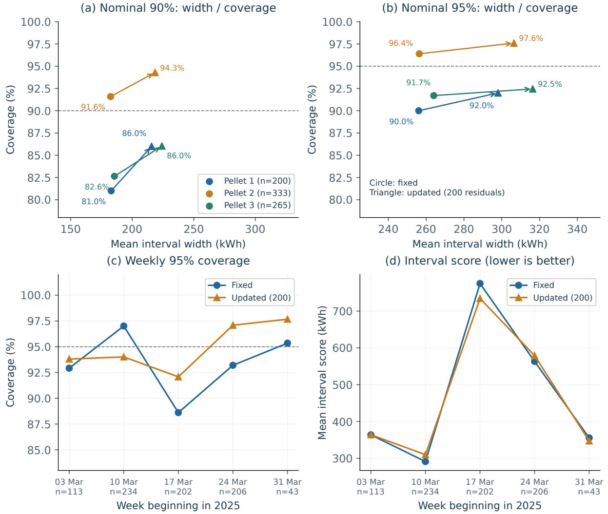
Figure S2: Coverage, width and interval score for the fixed calibration and the exploratory rolling update. (a,b) Line-specific coverage against mean interval width at nominal 90% and 95%; arrows connect fixed intervals (circles) to updated intervals (triangles). (c,d) Weekly 95% coverage and interval score, with sample sizes and partial weeks at the edges; dashed lines mark nominal coverage, and a lower interval score is better. Both policies use the same 798 fixed point predictions.
