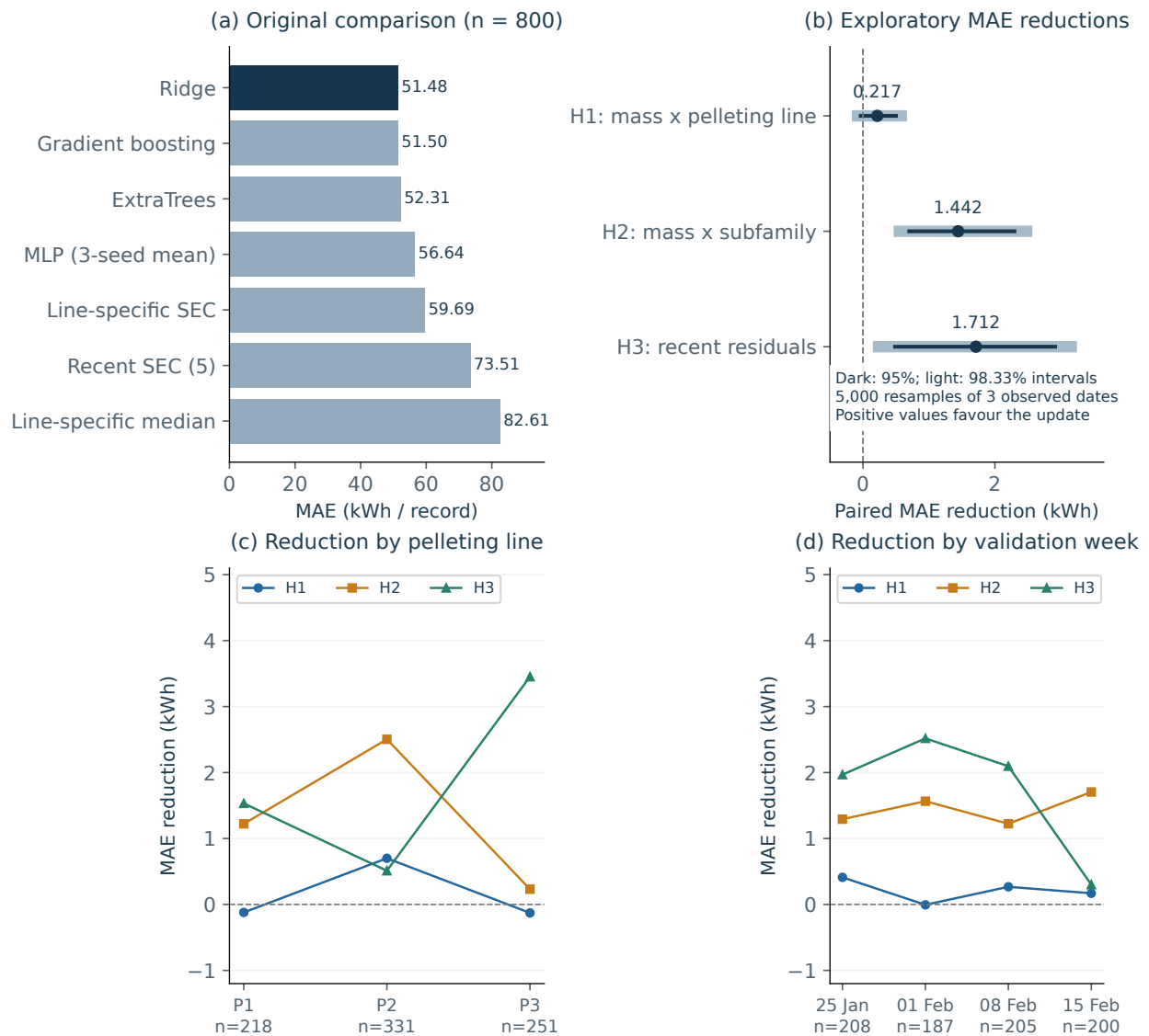
Figure S1: Development results and exploratory extensions. (a) MAE of the seven original methods on the 800 common development records. (b) Paired MAE reductions relative to Ridge for line-dependent mass effects (H1), product-dependent mass effects (H2) and recent-residual correction (H3), with 95% and multiplicity-adjusted 98.33% intervals. (c,d) Reductions by pelleting line and by validation week; positive values favour the extension.
