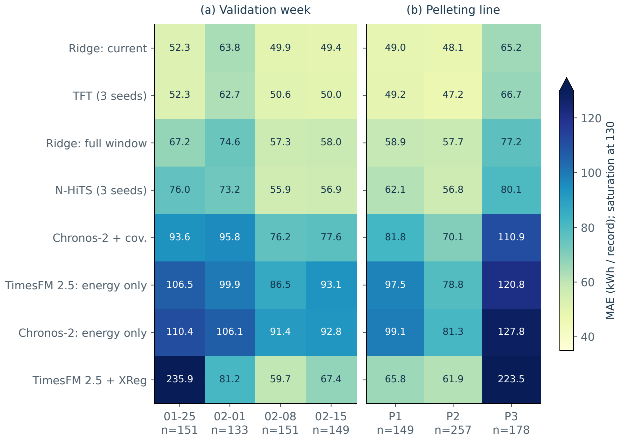
Figure S3: MAE by pelleting line and by validation week for the eight methods of the matched benchmark, in kWh per record; labels give the number of targets in each stratum. The colour scale ends at 130 kWh so that differences among the lower errors remain readable, while printed values preserve every result above that limit.
