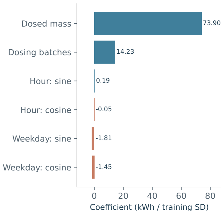
(c) Contributions across 798 records
