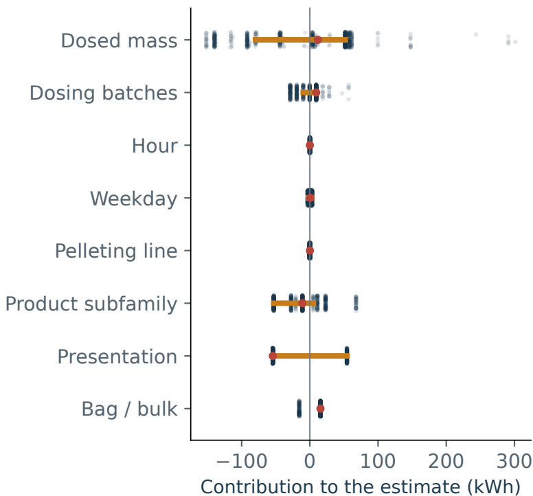
(c) Contributions across 798 records
