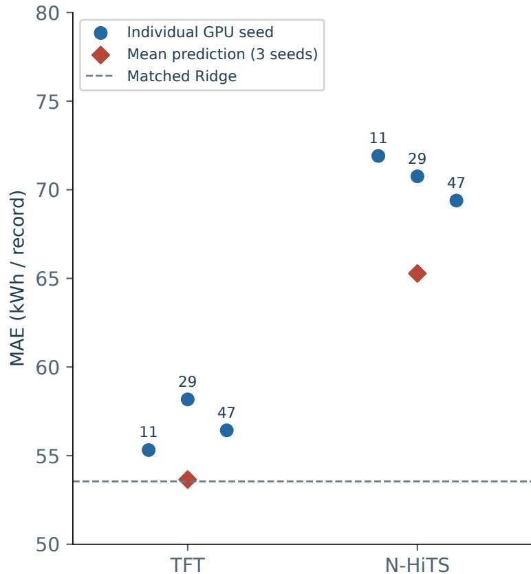
(b) Training seeds and ensemble
