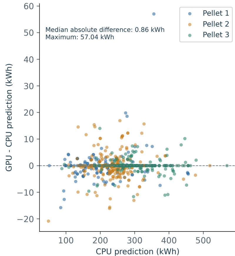
(a) Chronos-2: device differences
