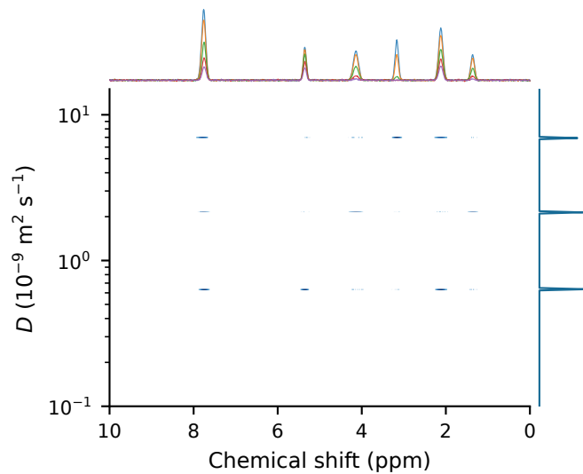
DOME-S
