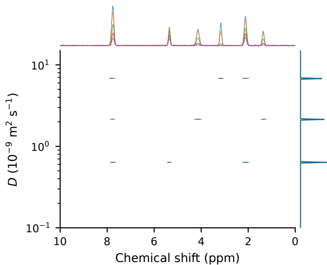
RAI-S
