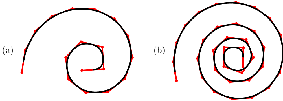
Figure 5: Interpolation of polygonal spirals, via De Casteljau's algorithm, derived from the Bill Picture. Comparison between a one-segment (a) and two-segment shift (b), with nested regular polygons from triangle to icosagon.
