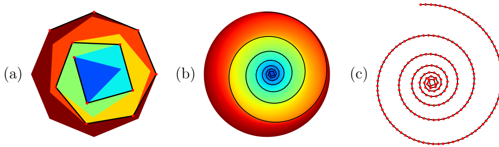
Figure 4: Nested regular polygons and emerging polygonal spiral: (a) from triangle to octagon, (b) from triangle to hectagon, and (c) highlighting the spiral-like evolution.
