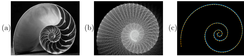
Figure 8: Comparison between the Nautilus shell and the figure obtained by combining the parameters from Figures 12.b and 12.c. An overlay of the logarithmic spiral with a ratio \sqrt{\varphi} \approx 1.27 (in orange) and the Bézier curves (in blue).
