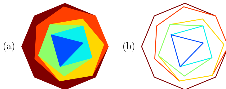
Figure 1: Filled (a) and contour representation (b) of the Bill Picture.
