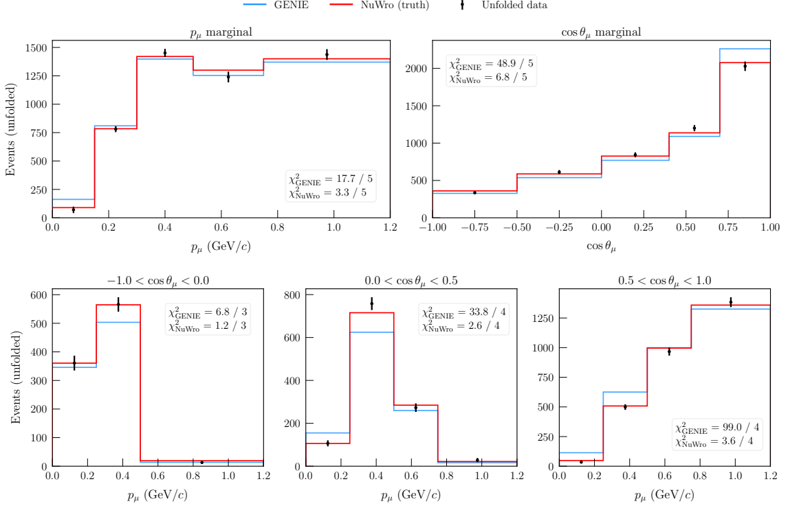
Figure 6. Unfolded event distributions for the realistic fake-data study. The GENIE (blue) and NuWro (red) truth-level predictions are smeared through the additional smearing matrix A_C for comparison with the unfolded fake data (points with propagated uncertainties). Per-block \chi^2 values are annotated in each panel.
