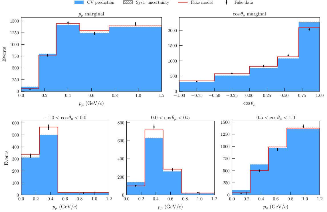
Figure 5. Reconstructed-space event distributions for the realistic fake-data study. The GENIE CV prediction (filled histograms) and systematic uncertainty bands (shaded) are compared to the NuWro prediction (red line) and a 5,000-event NuWro pseudo-data realization (points with statistical error bars). The top row shows the p_\mu and \cos \theta_\mu marginals; the bottom row shows the three \cos \theta_\mu slices of the 2D block.
