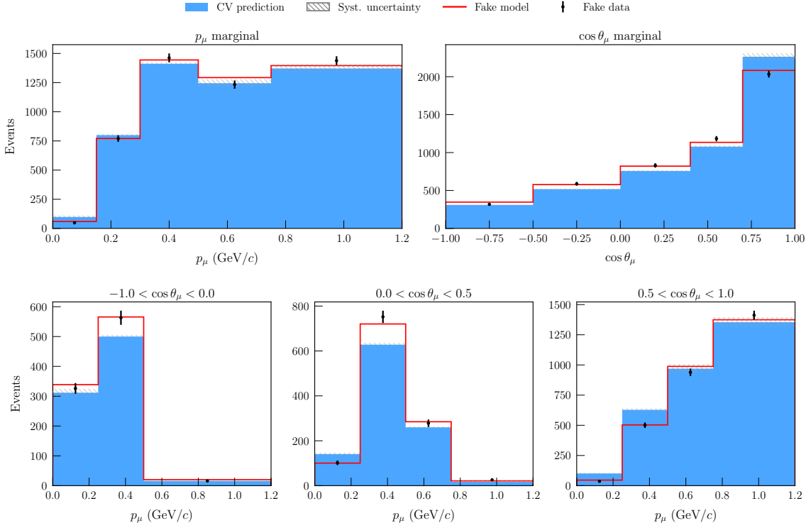
Figure 6. Reconstructed-space event distributions for the realistic fake-data study. The GENIE CV prediction (filled histograms) and systematic uncertainty bands (shaded) are compared to the NuWro prediction (red line) and a 5,000-event NuWro pseudo-data realization (points with statistical error bars). The top row shows the p_\mu and \cos \theta_\mu marginals; the bottom row shows the three \cos \theta_\mu slices of the 2D block.
