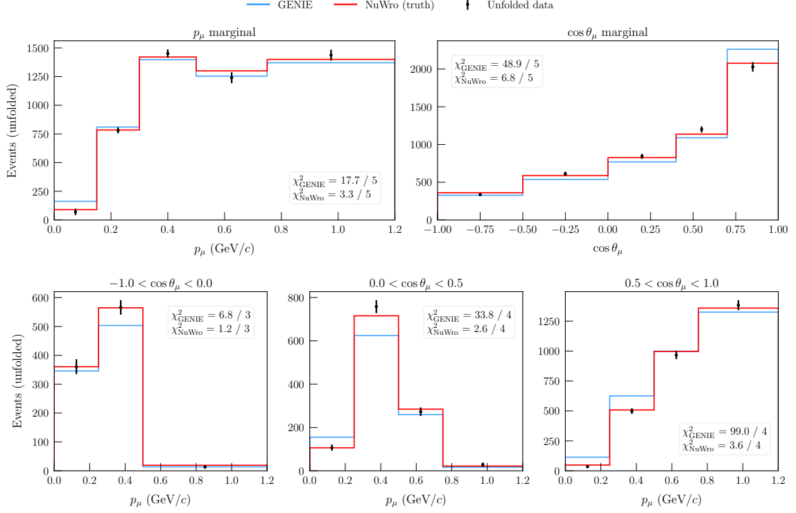
Figure 7. Unfolded event distributions for the realistic fake-data study. The GENIE (blue) and NuWro (red) truth-level predictions are smeared through the additional smearing matrix A_C for comparison with the unfolded fake data (points with propagated uncertainties). Per-block \chi^2 values are annotated in each panel.
