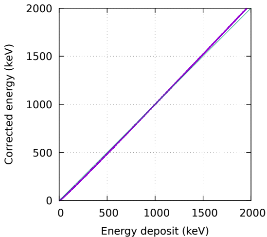
Electron Birks-Cerenkov corrected energy E_{\text{ref}}=1 \text{ MeV}
