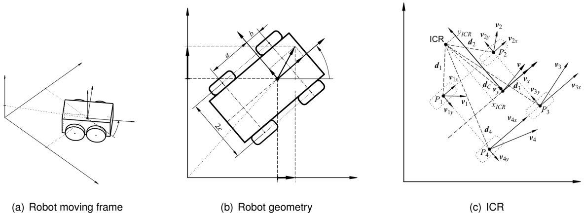
Figure 3.1: Car-like robot kinematics [14]
