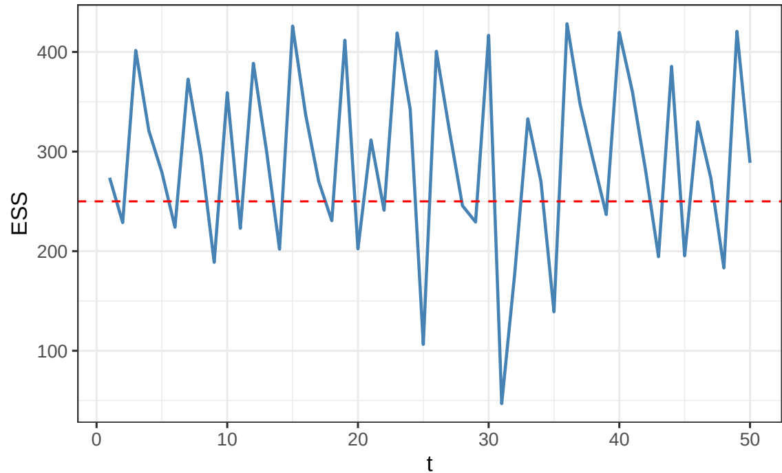
Effective sample size (N=500, eps=0.01)
