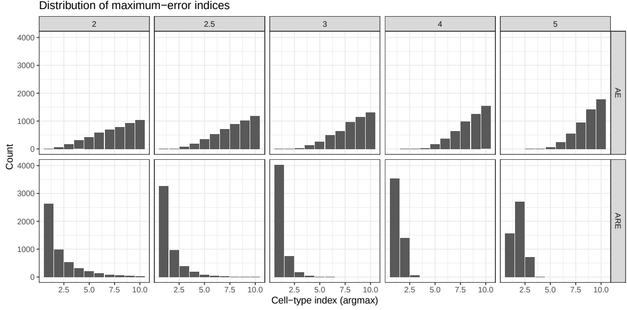
Figure 3: Argmax histograms by alpha and metric for maximum-error indices.
