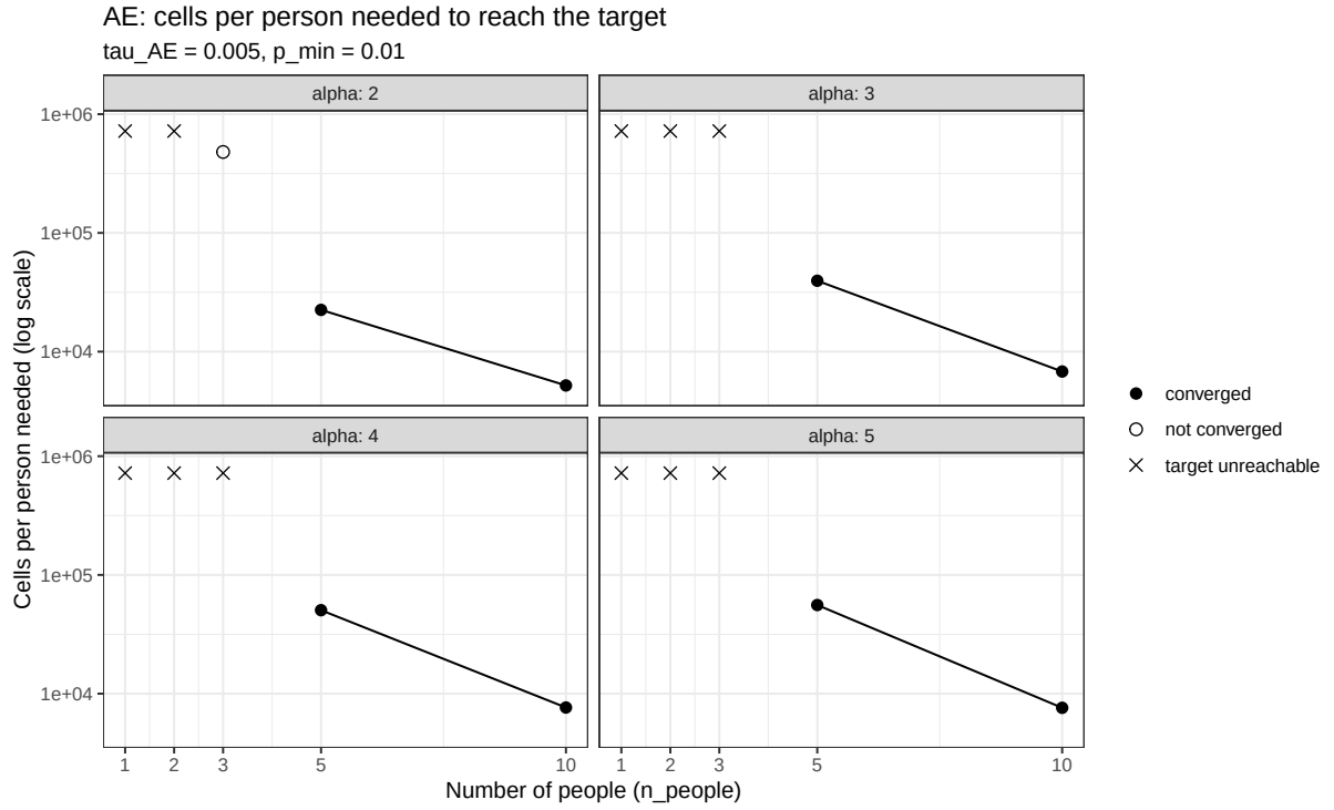
Figure 6: Cells per person needed to reach the 95% AE success target at \tau_{AE} = 0.005 (log scale), versus the number of people N . One panel per \alpha . An open marker means the solver did not converge; \times at the top means the target cannot be reached.
