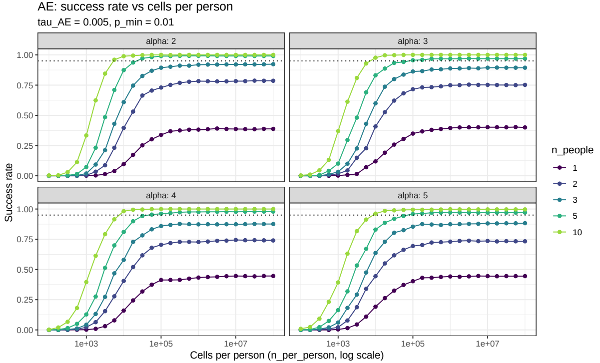
Figure 4: AE success rate versus cells per person (log scale) at \tau_{AE} = 0.005 . Success rises with cells per person and then reaches a plateau.
