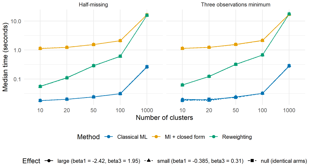
Figure 10: Median computation time per replicate (log scale).
