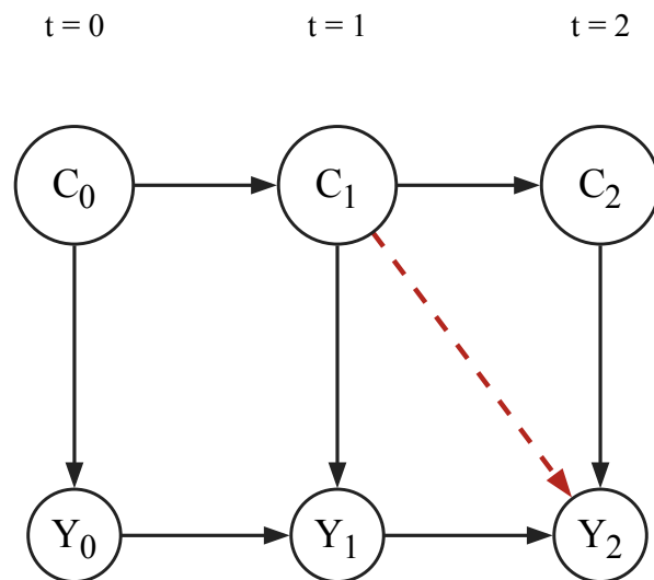
(b) Coarse quotient: C = \{X, Z\}
