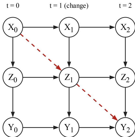
(a) Fine graph
