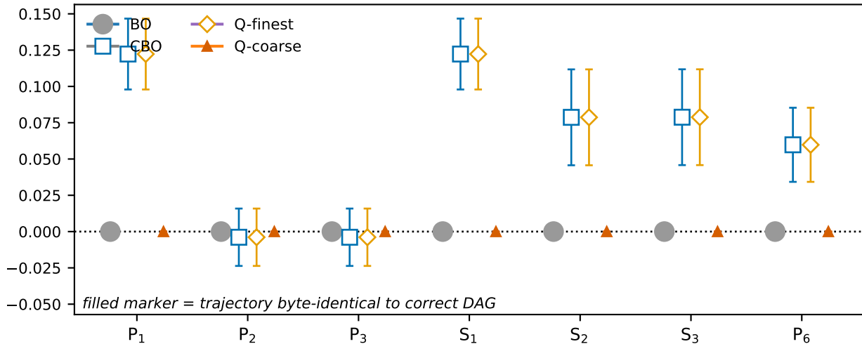
Quotient-invisible edits (Prop. 2: guarantee holds)
