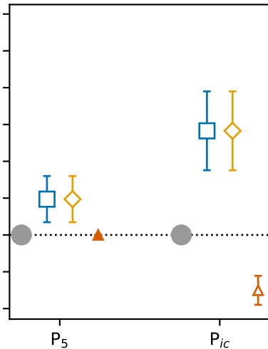
Quotient-visible edits (guarantee out of scope)
