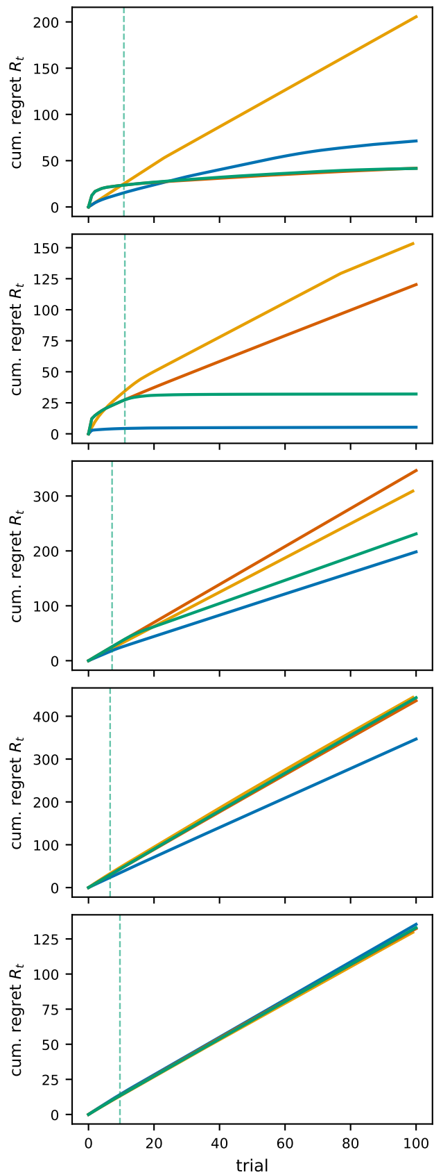
cumulative regret
