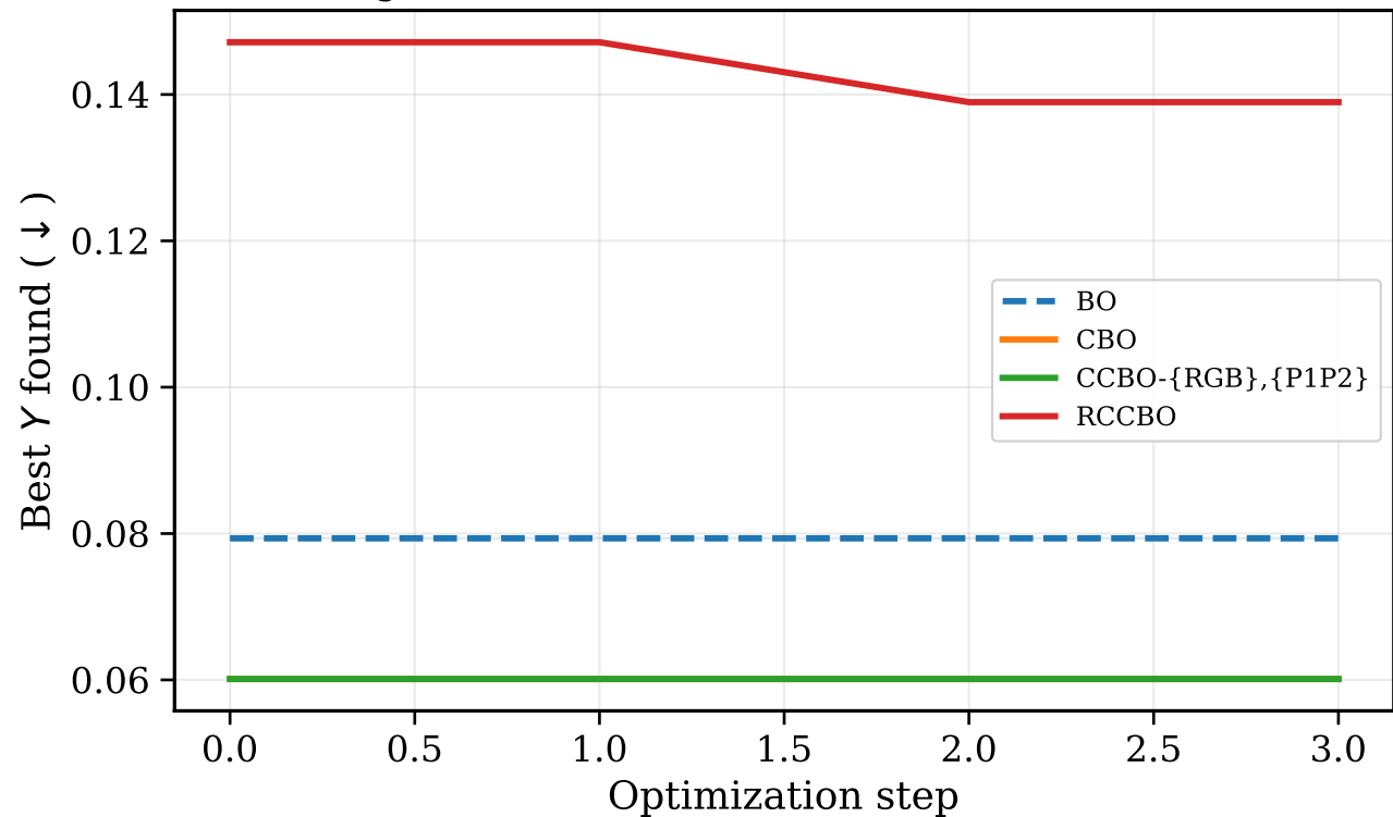
LightTunnel: BO vs CBO vs CCBO vs RCCBO
