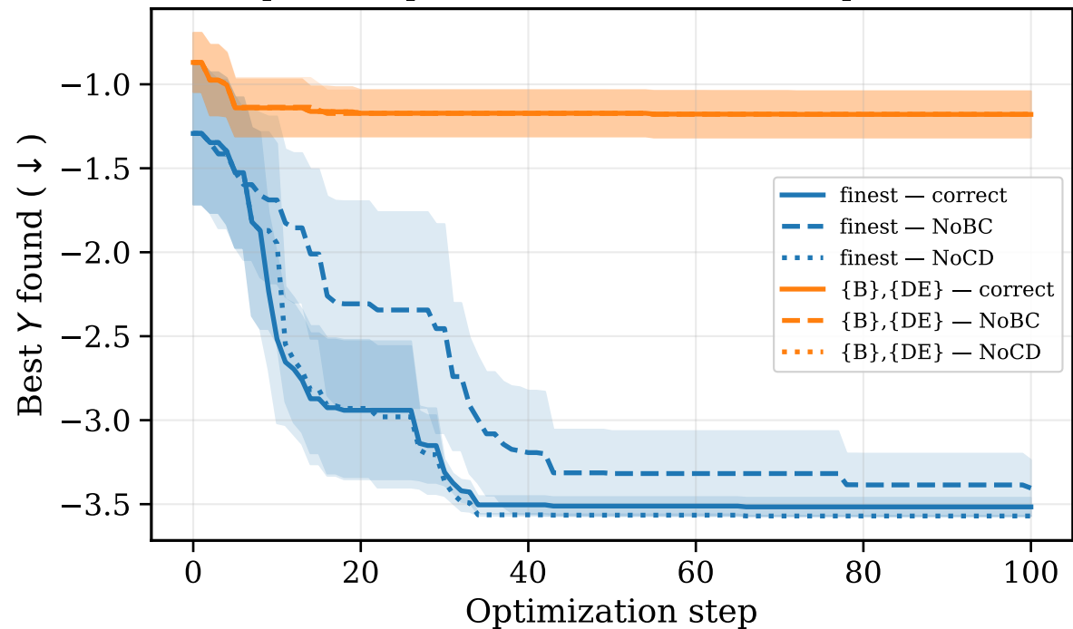
CompleteGraph: robustness under misspecification
