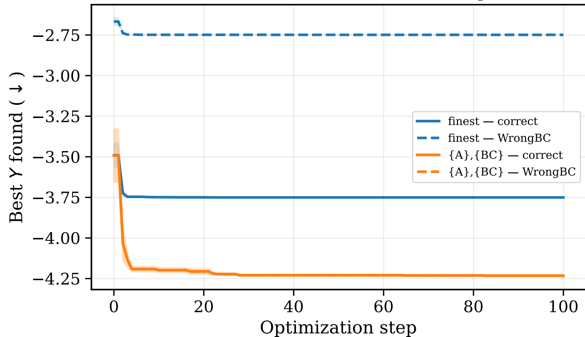
ConfoundedCluster: robustness under misspecification
