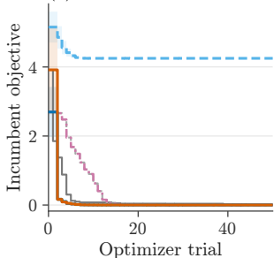
(a) ParallelParent
