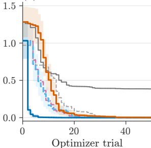
(b) FrontDoor
