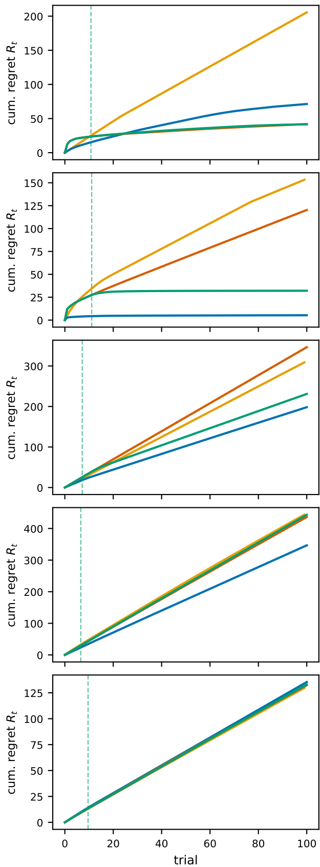
cumulative regret
