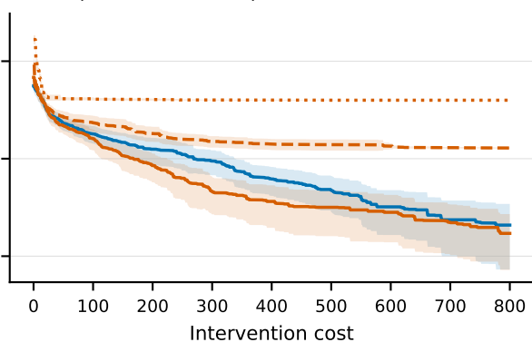
K3: drop A_1 \leftrightarrow A_2 (biased prior)
