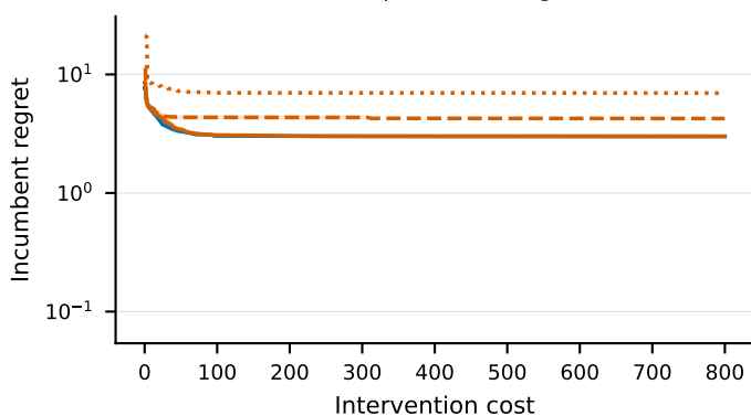
K2: delete D_1, D_2 \rightarrow Y (quotient changed)
