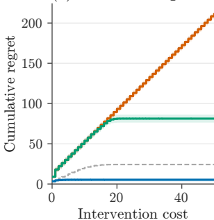
(b) Cumulative regret
