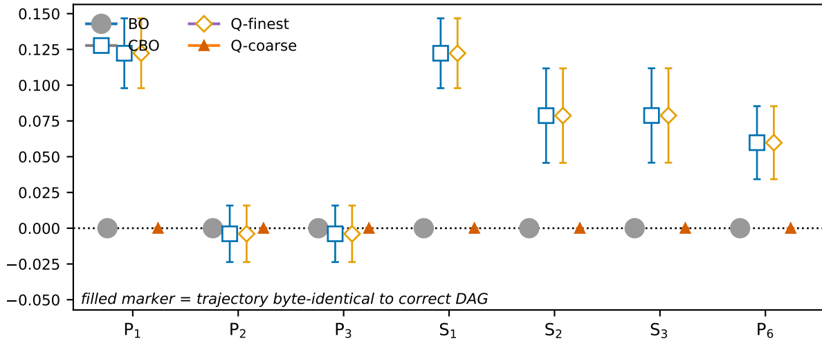
Quotient-invisible edits (Prop. 2: guarantee holds)
