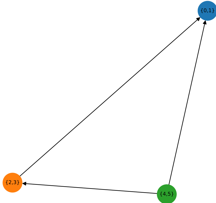
True condensation (ground truth) [Tarjan's on true graph → 3 blocks]
