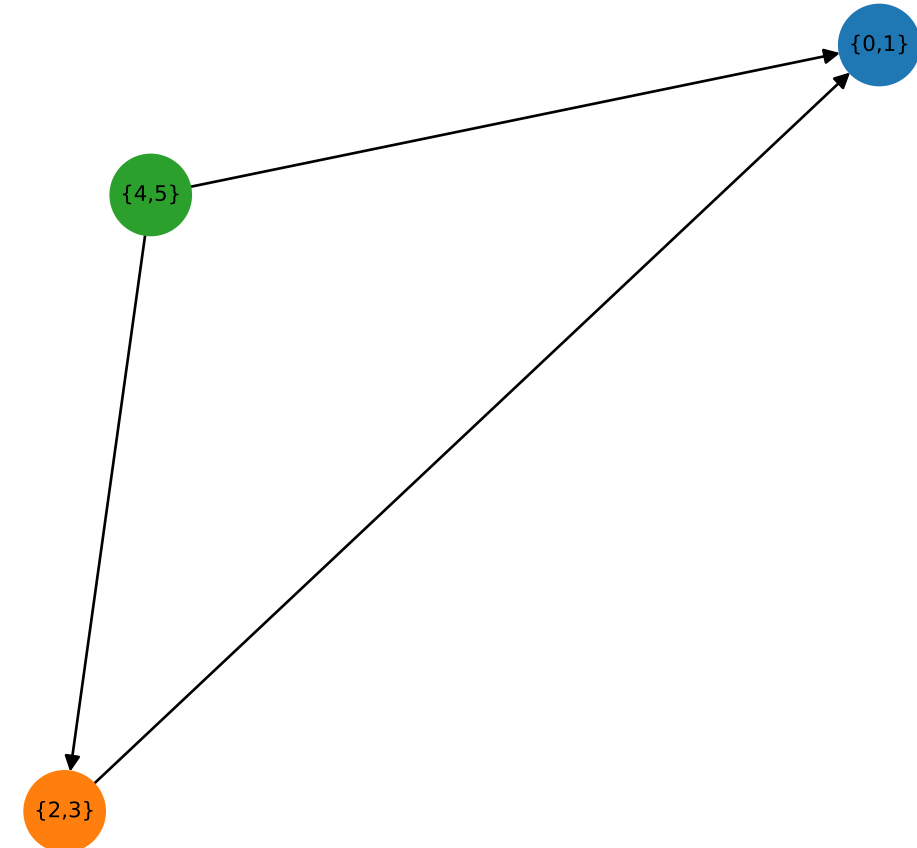
OICA estimate (8,000 obs. samples) [Tarjan's on ICA support → 3 blocks found]
