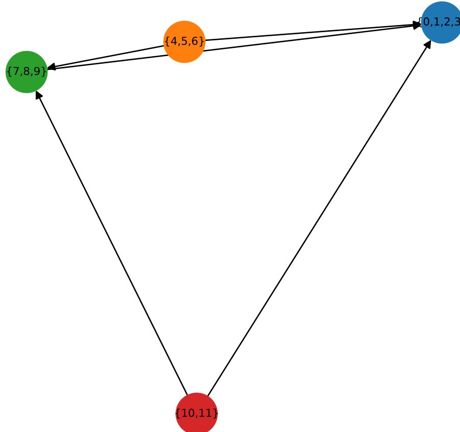
True condensation (ground truth) [Tarjan's on true graph → 4 blocks]
