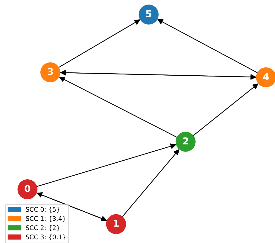
True DG (nodes coloured by SCC)
