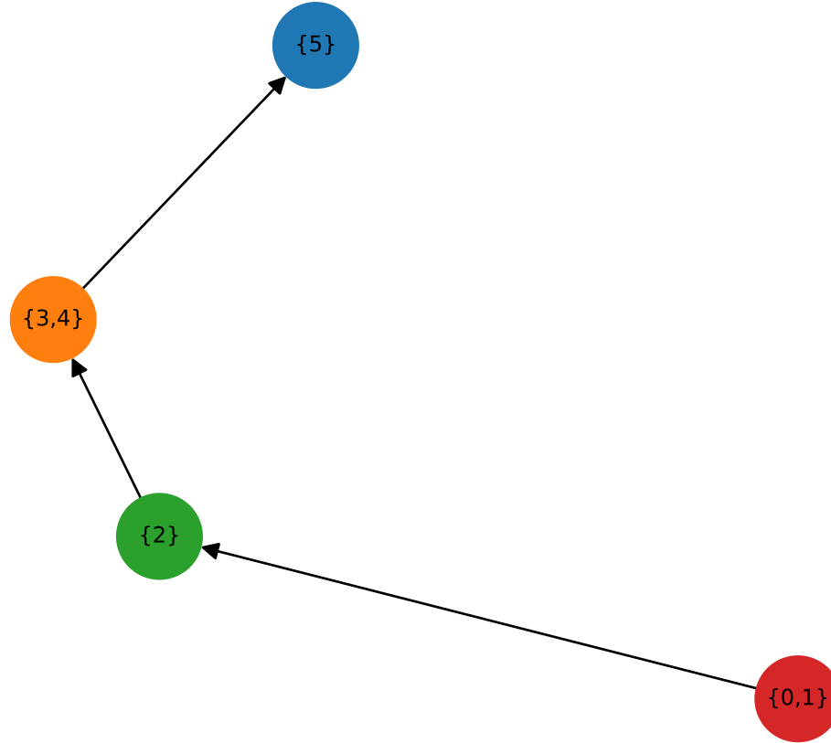
True interventional coarsening G^I
