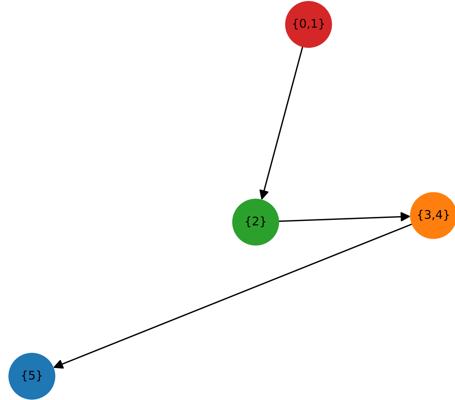
Discovered partition DAG (RePaRe-Cycle)
