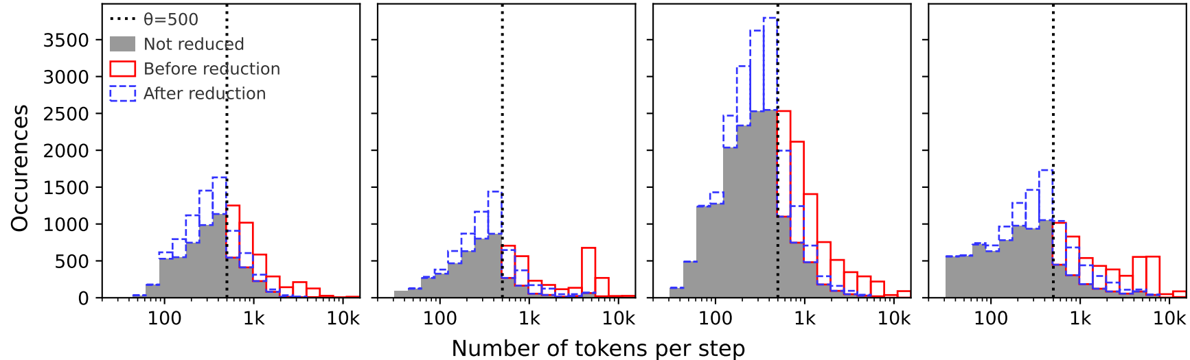
SbV+Claude
