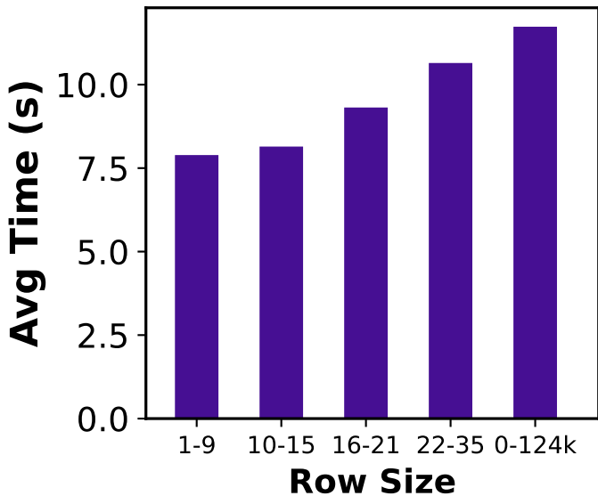
Synth-Spider
