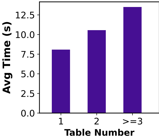
Synth-Spider
