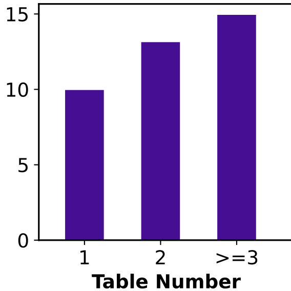
Synth-Bird
