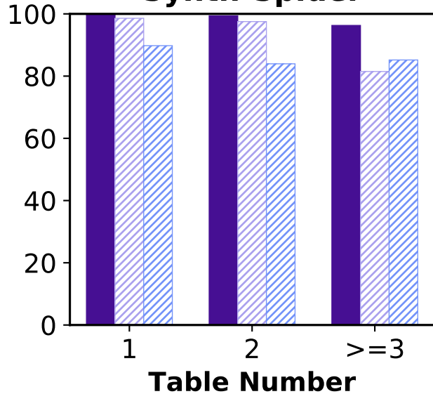
Synth-Spider
