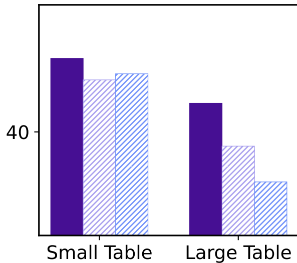
Parrot
