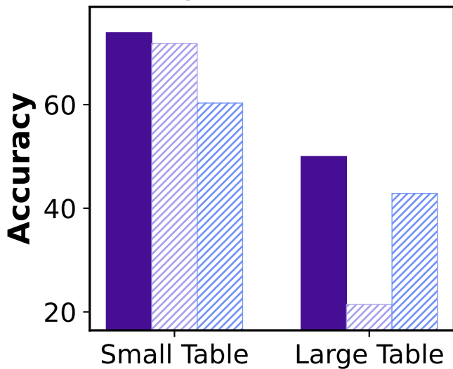
Synth-Spider
