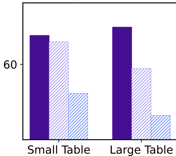
Synth-Bird
