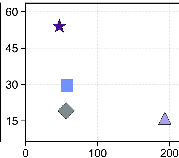
NL2SQL-Bird
