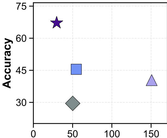
NL2SQL-Spider
